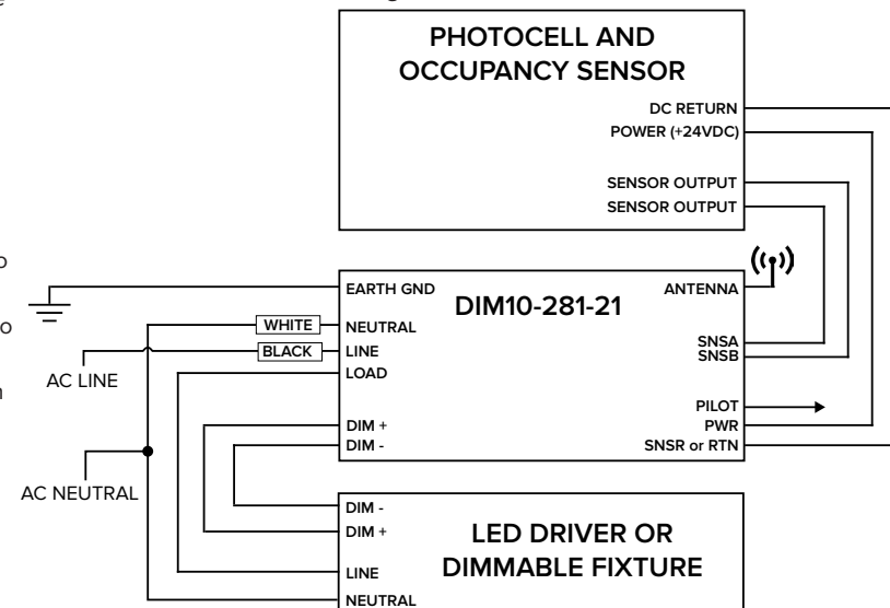
Figure 2 - Wiring Diagram
