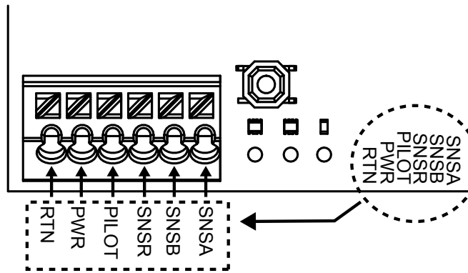
Figure 3 - Terminal Block Identifiers
